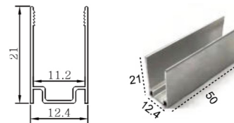
Aluminum clips
