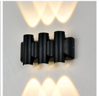
GB815A-3 Lamp:LED 6×1W Size:170×90×42
