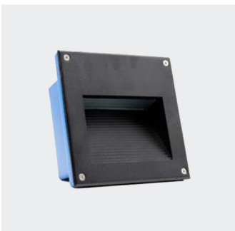
GQ5099 Lamp:LED 1×6W Size:160×160×80
